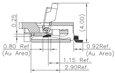
SECTION Q-Q SCALE 2:1
