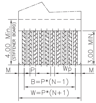
APPLICABLE FPC/FFC DIMENSION THICKNESS:T=0.30±0.05
