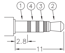
φ2.5mm SPECIAL MATE PLUG
