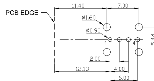
SUGGESTED PCB LAYOUT TOP VIEW
