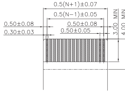
APPLICABLE FPC/FFC DIMENSION THICKNESS: T=0.30±0.05
