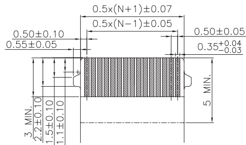
APPLICABLE FPC/FFC DIMENSION THICKNESS: T=0.30±0.05
