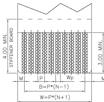
APPLICABLE FPC/FFC DIMENSION THICKNESS:T=0.30±0.05
