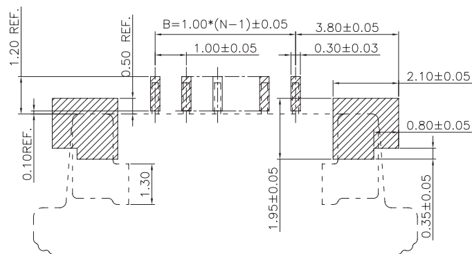
RECOMMEND PCB LAYOUT SIZE
