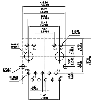
RECOMMENDED PCB LAYOUT TOP VIEW TOLERANCE: ±0.05mm PCB THICKNESS: 1.60±0.05mm
