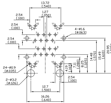
RECOMMENDED PCB LAYOUT TOP VIEW THICKNESS=1.60mm
