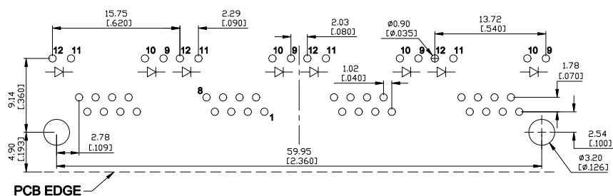
SUGGESTED PCB LAYOUT TOP VIEW
