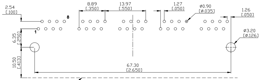
SUGGESTED PCB LAYOUT TOP VIEW
