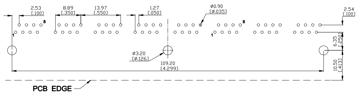
SUGGESTED PCB LAYOUT TOP VIEW
