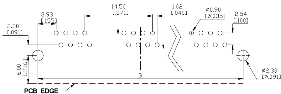
SUGGESTED PCB LAYOUT TOP VIEW
